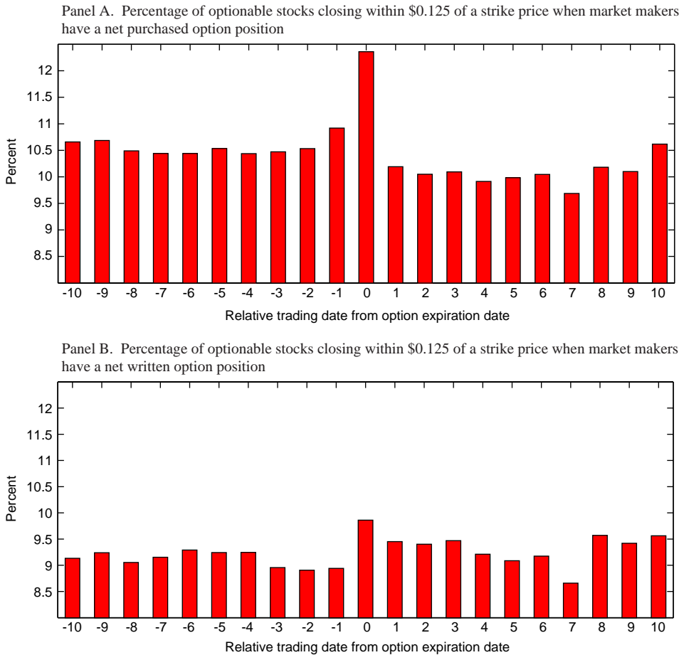
Fig. 6. Percentage of optionable stocks closing within $0.125 of an option strike price as a function of the number of trade dates before or after an option expiration date, for subsets of stock–expiration date pairs in which market makers have net purchased or net written positions on the closest to expiration options with strike price nearest to the closing stock price. Expiration Fridays are trade date ‘0’ relative to the option expiration date, the Thursdays before are trade date ‘-1’ relative to the option expiration date, the Mondays after are trade date ‘1’ relative to the option expiration date, etc. For each trade date relative to the expiration date, the plots show the percentages of stocks that close within $0.125 of a strike price of an option listed on the stocks. The data period is January 1996–December 2001.
